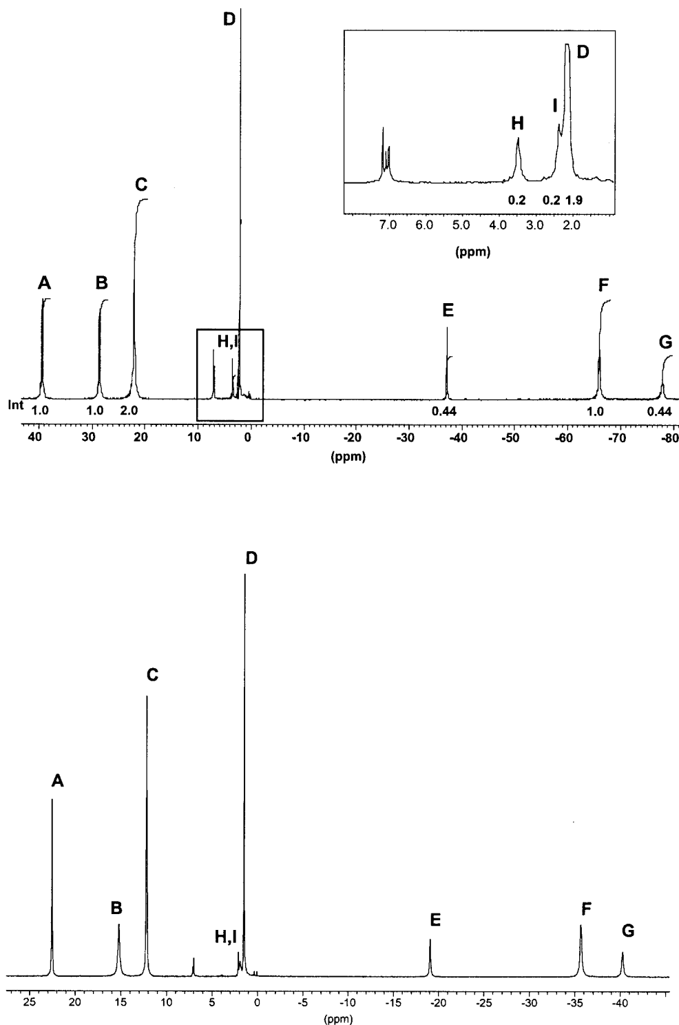
Figure 2. Representative variable-temperature ^1\text{H} NMR spectra of [\text{Nd}(\mu_3\text{-OtBu})_2(\mu_2\text{-OtBu})_2(\text{OtBu})\text{Mg}_2(\text{CH}_2\text{SiMe}_3)_2(\text{THF})] ( 4 ) in [\text{D}_8] -toluene; top: -80\text{ }^\circ\text{C} ; bottom: 0\text{ }^\circ\text{C} (I denotes residual toluene resonance and/or a signal from 4 )
