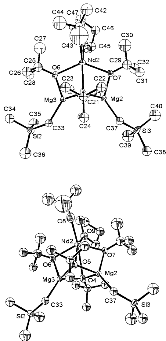
Figure 1. Two views of the molecular structure of [\text{Nd}(\text{THF})(\mu_3\text{-OtBu})_2(\mu_2\text{-OtBu})_2(\text{OtBu})\text{Mg}_2(\text{CH}_2\text{SiMe}_3)_2] ( 4 ); ellipsoids are drawn at the 40% probability level and hydrogen atoms omitted for clarity
